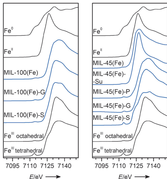
Figure 2. Normalized Fe K-edge XANES spectra of selected solutions, gels, and final crystalline samples of MIL-100(Fe) (left) and MIL-45(Fe) (right) along with references compounds (Fe metal–Fe 0 , FeSO 4 ·7H 2 O–Fe II , Fe 2 (SO 4 ) 3 ·5H 2 O–Fe III octahedral and FePO 4 ·2H 2 O–Fe III tetrahedral). The spectra are displaced vertically for clarity. In the case of MIL-45(Fe), the stage in the synthesis where the iron is reduced manifests as a shift of the absorption edge towards lower energies.
